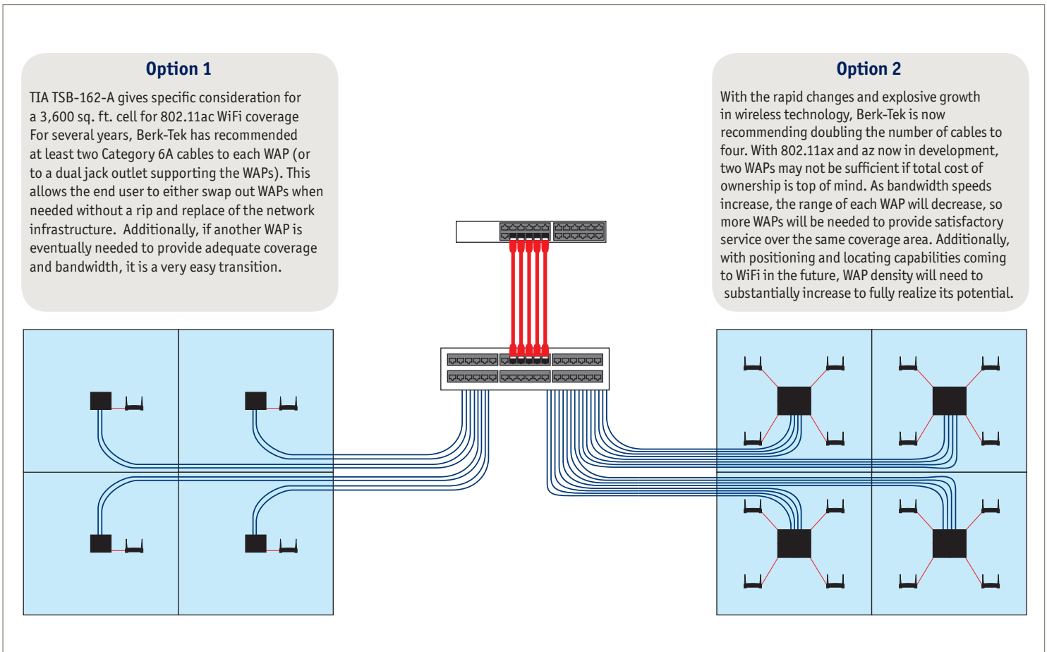
Figure 5: Examples of Typical Zone Cabling Designs
