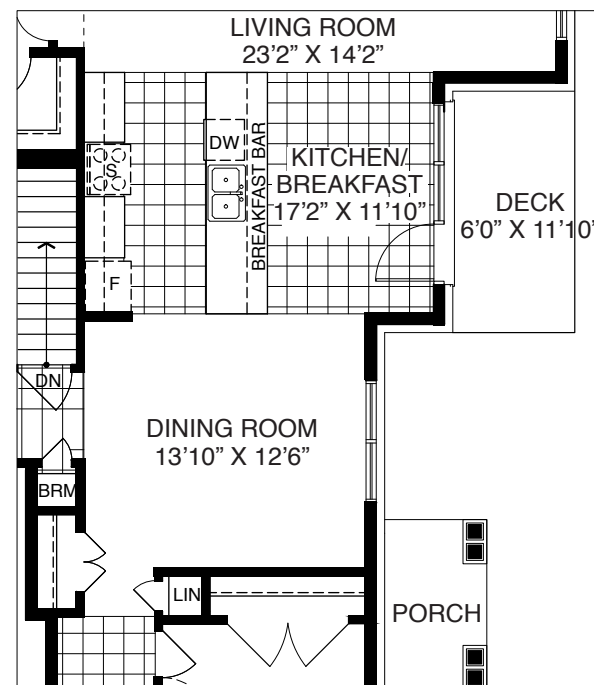
OPT. MAIN LEVEL LOT 21
