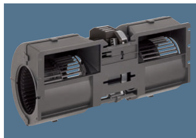
EC dual centrifugal blowers: for maximum performance with the smallest installa- tion space; easy to control and extremely quiet.
