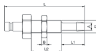
Panel Mount Hose Barb Plug
