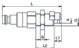
Panel Mount Plastic Hose Connect. Plug
