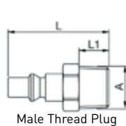
Male Thread Plug
