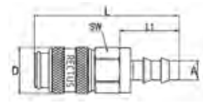
Push-Lock Hose Barb Coupler
