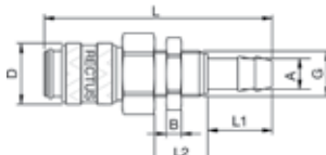
Panel Mount Hose Barb Coupler
