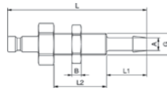
Panel Mount Hose Barb Plug
