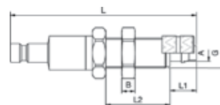
Panel Mount Plastic Hose Connect. Plug
