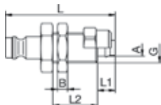
Panel Mount Plastic Hose Connection Plug
