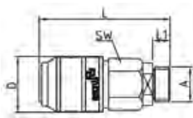
Male Thread Coupler Straight Sleeve
