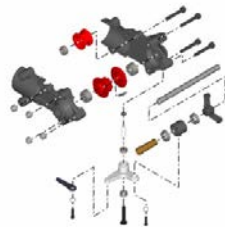
Exploded View
