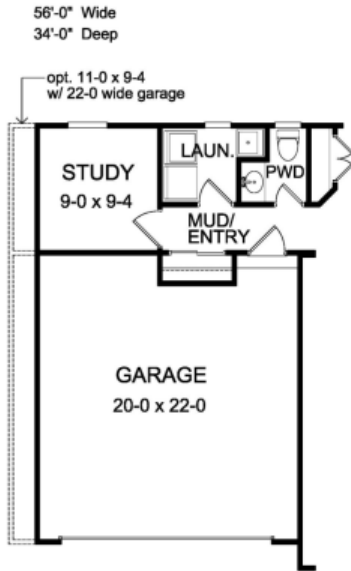
OPT. W/ STUDY (9-0 x 9-4 ) Additional = 107 Sq. Ft. (11-0 x 9-4 ) Additional = 127 Sq. Ft.
