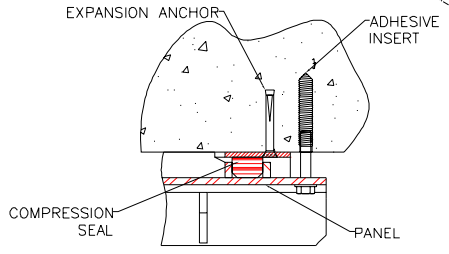
JAMB SECTION VIEW SECTION A-A
