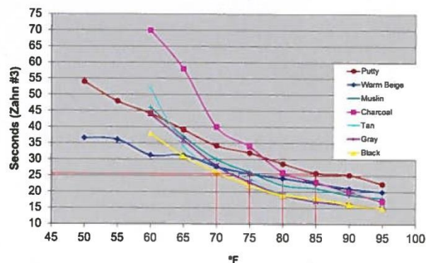
Figure 1: Relationship between Paint Viscosity and Temperature 3
