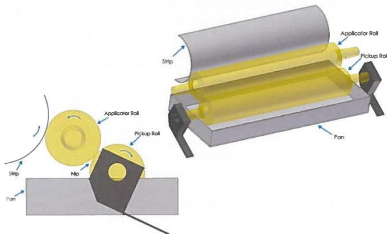
Figure 2: Typical 2-Roll Reverse (Indirect) Coating Configuration
