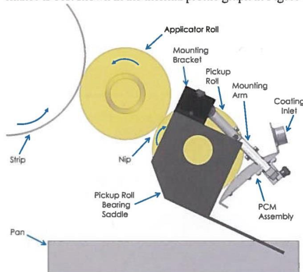
Figure 10: PCM Configuration
