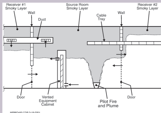
Figure 1. Fire Model Illustration
