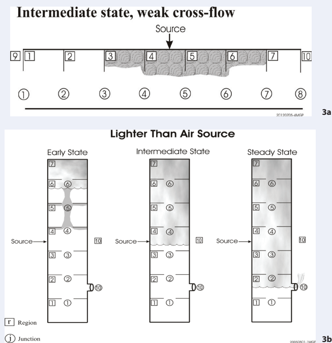
Figure 3. FATE Calculations
