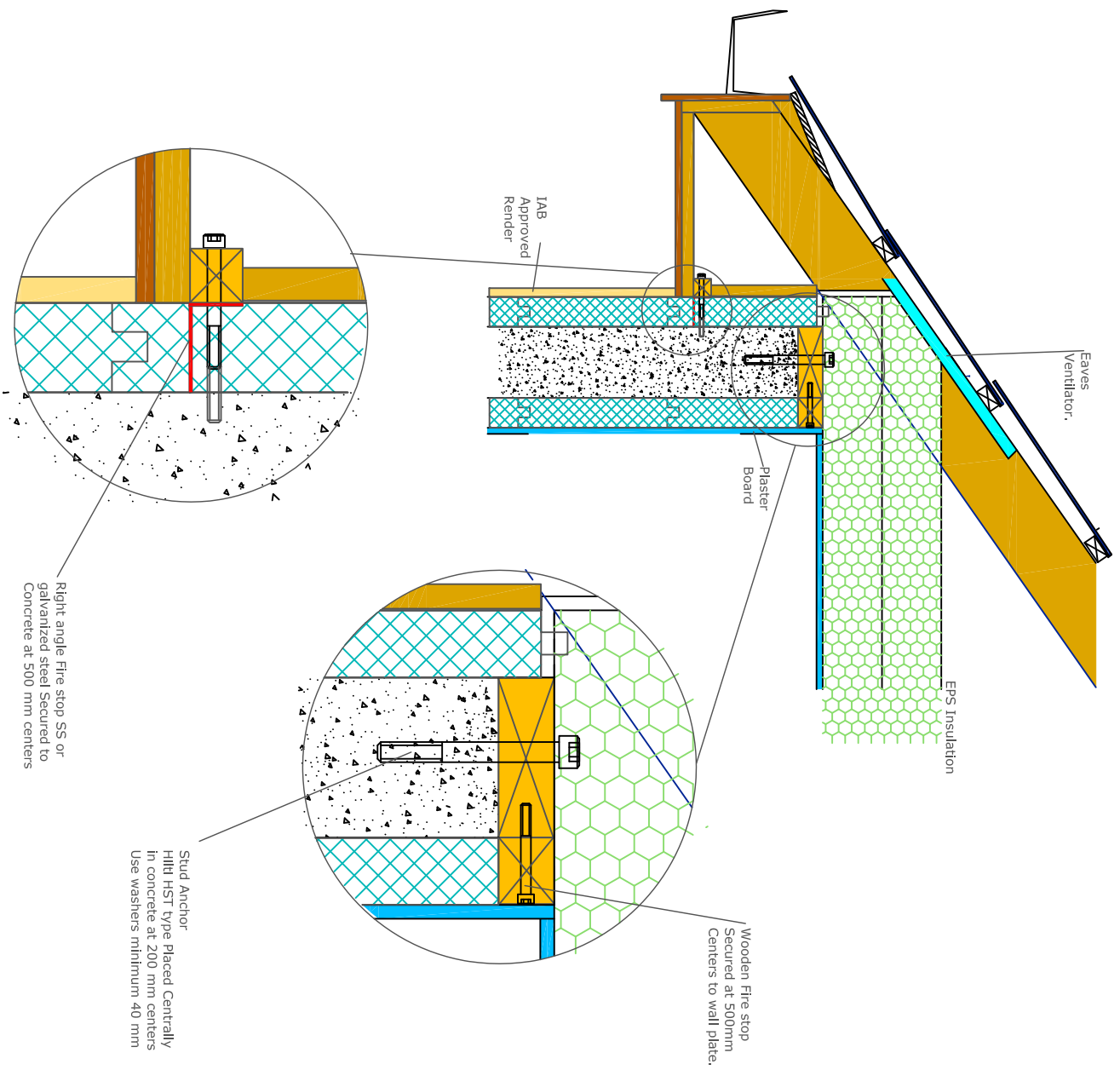
KORE Roof Plate & Soffit FIG 15.
