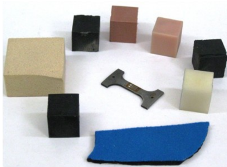
Figure 1: Components and materials of the WorldSID 50 dummy
