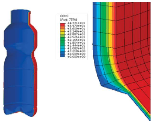
Abaqus software example of the mass diffusion FEA method in an oxygen concentration analysis.
