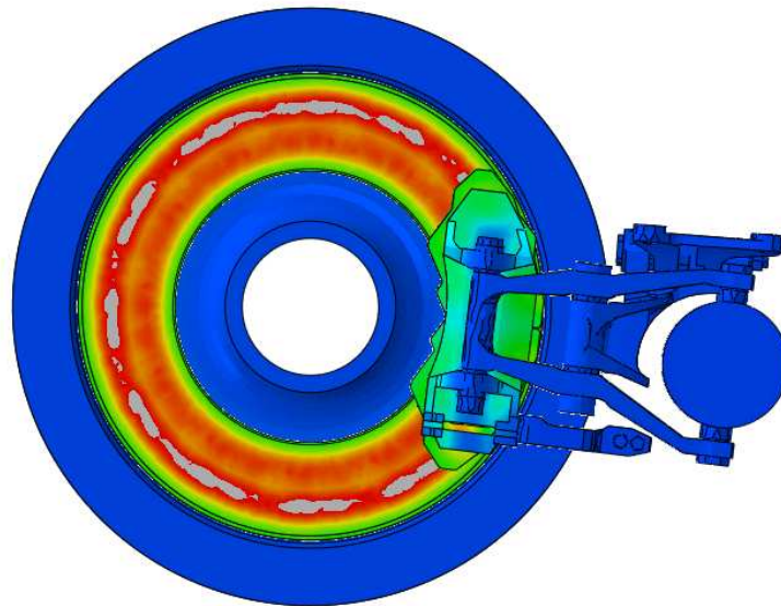
Figure 5. Temperature contours of experiment and analysis
