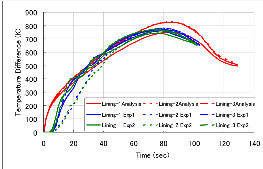
Figure 8. Temperatures of the linings (350km/h)
