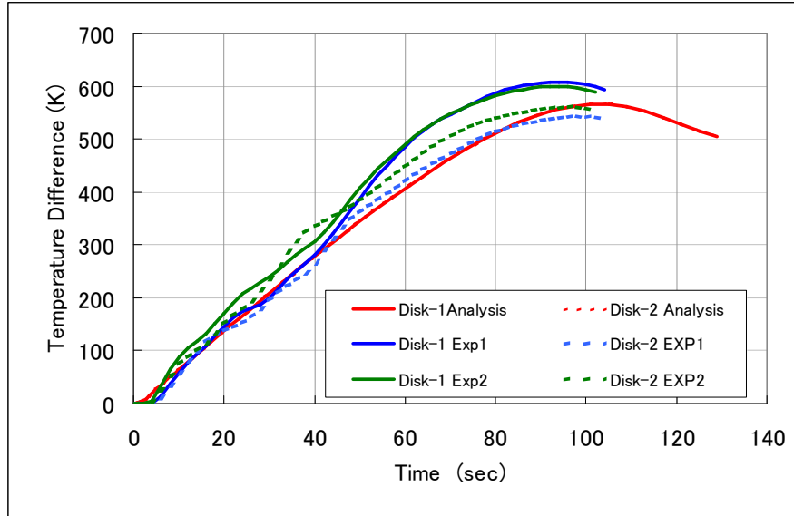
Figure 6. Temperatures of the discs (350km/h)
