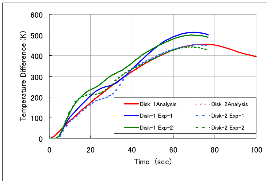
Figure 7. Temperatures of the discs (300km/h)
