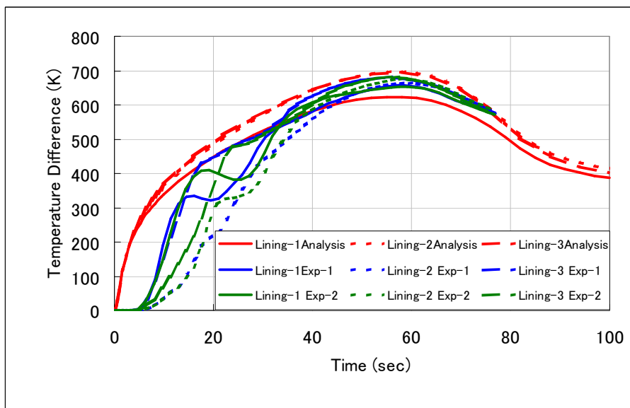
Figure 9. Temperatures of the linings (300km/h)
