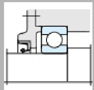
Contacting Single Lip Oil Seal Design
