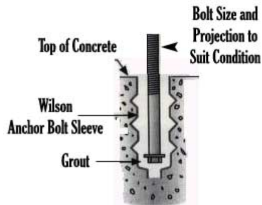
Figure 2 - Grout Pocket
