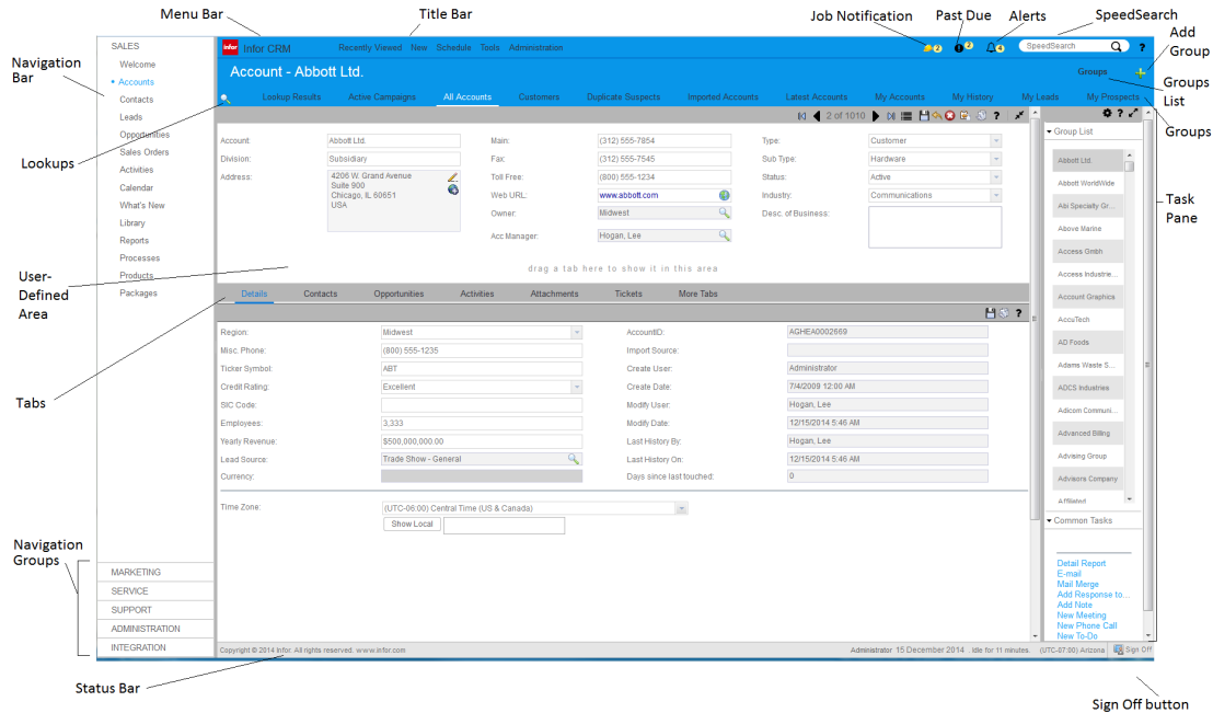
Figure 1 Infor CRM Web Client Workspace
