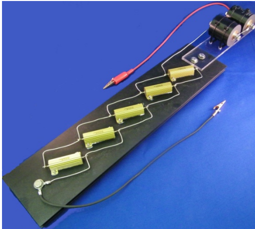
Antenna Simulator
