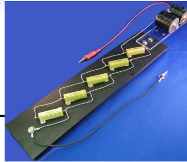
Antenna Simulator
