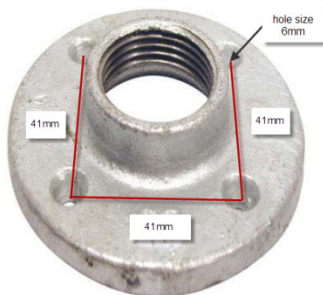
MR5 Flange
