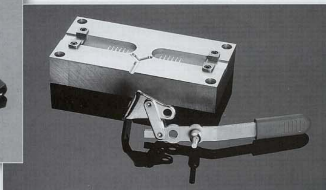
INJECTION MOLDING
