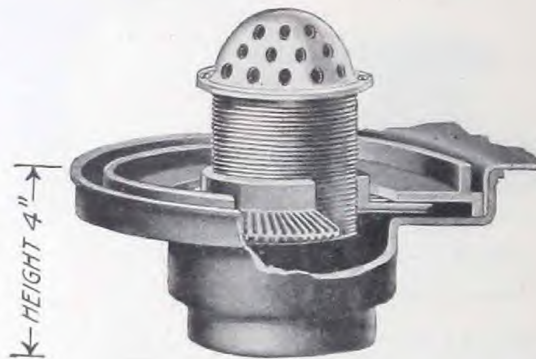
No. 135 Urinal Drain Head—Outlet 2 or 3 Inches
