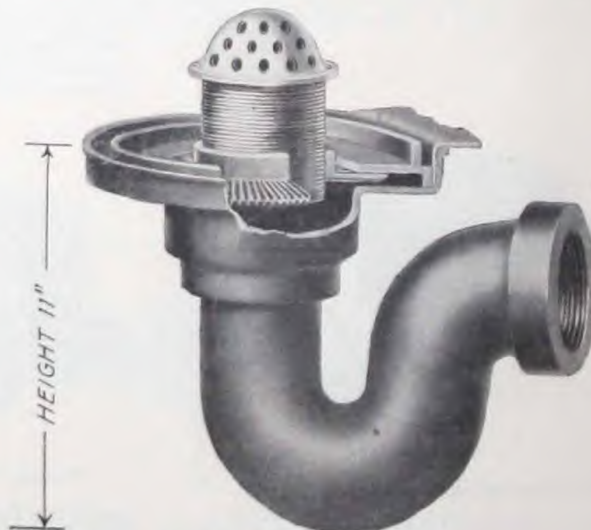
No. 70-135 Urinal Trap—Outlet, 3 Inches. Also furnished with Flat Strainer
