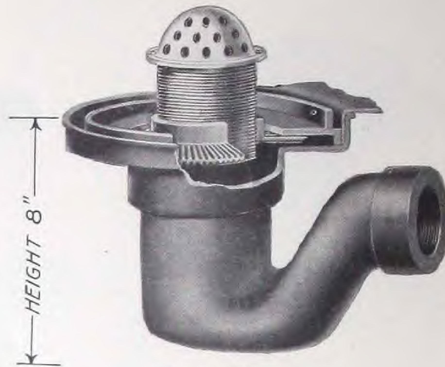
No. 126-135 Urinal Trap—Outlet, 2 Inches
