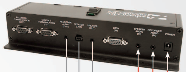
Control Box
