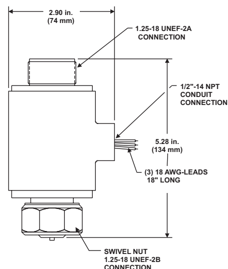
Figure 1. Assembly Drawing
