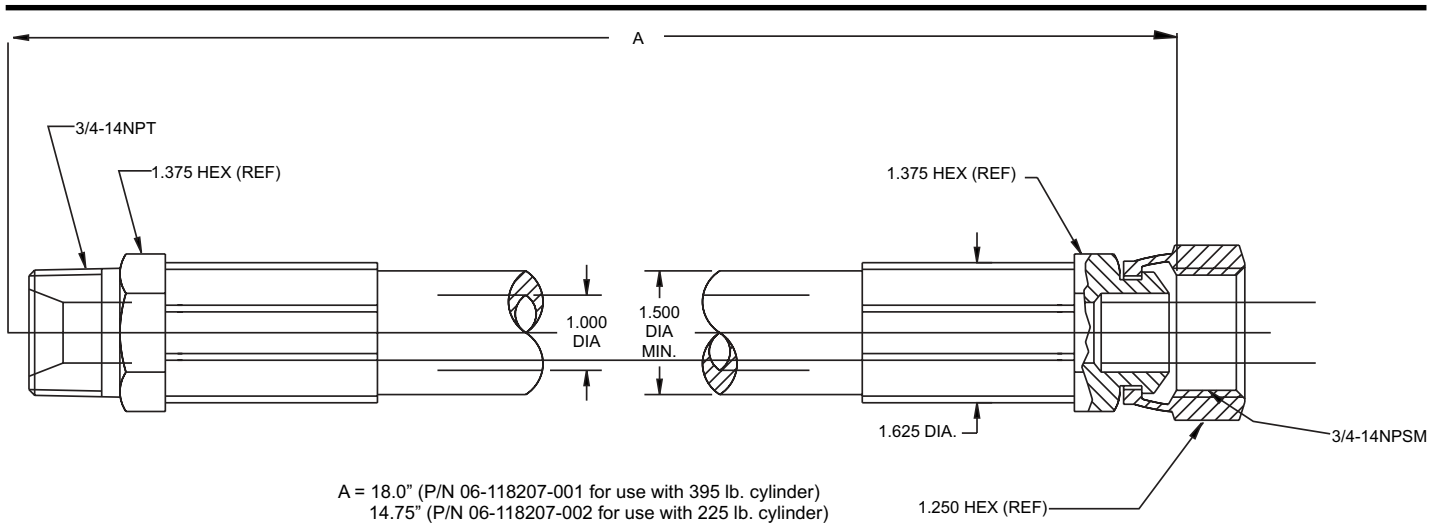
Figure 1. Nitrogen Transfer Hose
