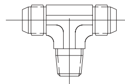
MALE BRANCH TEE 1/8" NPT X 5/16" TUBING P/N 6992-0505
