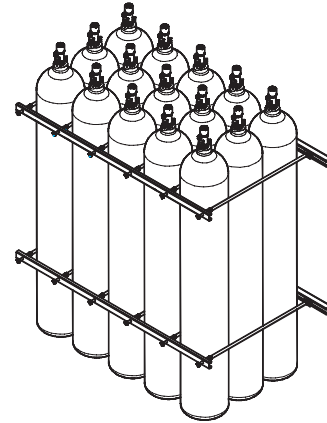
15 Cylinder, Triple Row Racking Assembly
