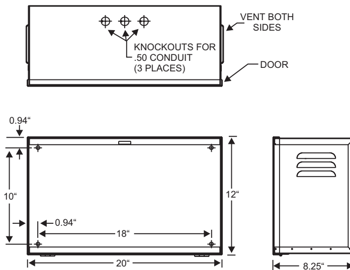
Figure 1. Battery Enclosure Diagram
