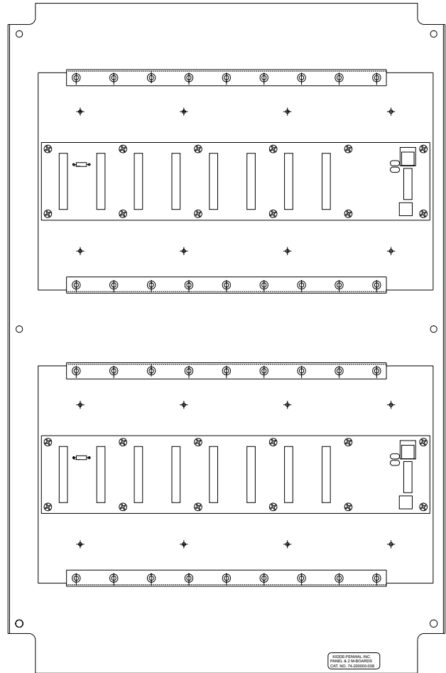
Figure 3. Two I/O Module Card Cages with Provisions for Two I/O Mother Boards (P/N 76-100000-008)
