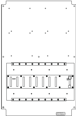
Figure 1. I/O Module Card Cage with Provisions for One I/O Mother Board and Four Power Supply Modules (P/N 76-100000-006)
