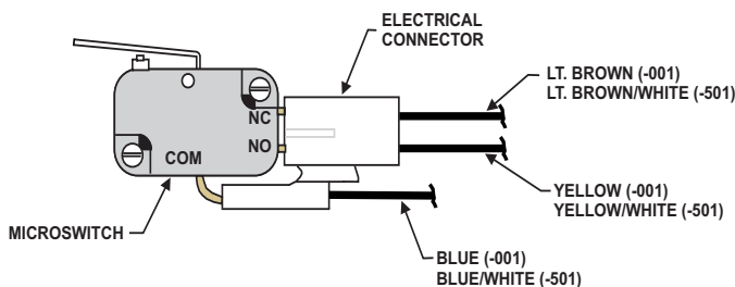
Figure 1. Quick Connect Microswitch
