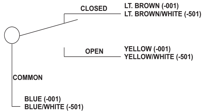
SWITCH POSITION WHEN XV CAM/FLAG IS IN 'RELEASED' POSITION
