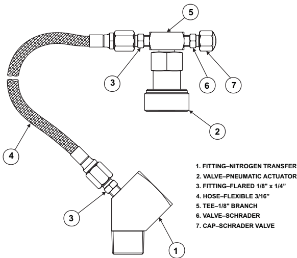
Figure 1. Actuation Kit Assembly
