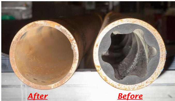
Decoating of 10 m stator tubes inside and outside
