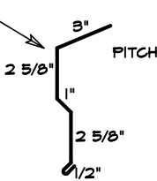
5a 2X6 EAVE
