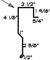
4a 2X6 GABLE
