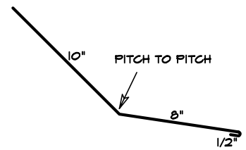
20b TRANSITION LOW HIGH
