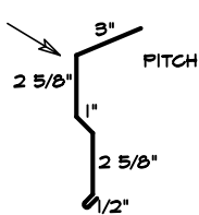
5a 2X6 EAVE
