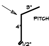
5b 2X4 EAVE
