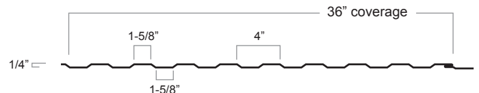
Platte River Panel (PRP) Profile *Wall Panel Only
