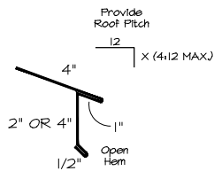
(5c) STYLE D EAVE
