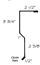
(10a) SIDEWALL
