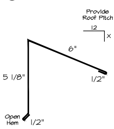
(5c) STYLE D EAVE
