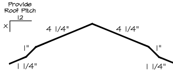
(1b) NON VENTED RIDGE CAP
