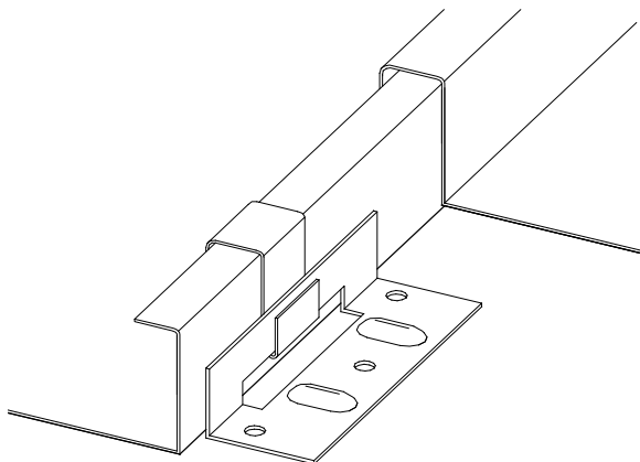
SLIDER CLIP
