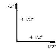
(14) INSIDE CORNER
