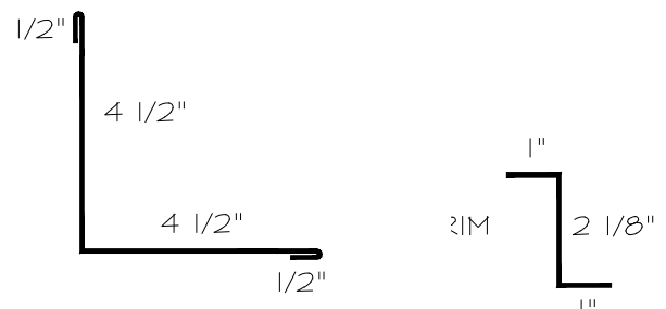
Inside Corner
