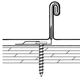
180° SEAM
