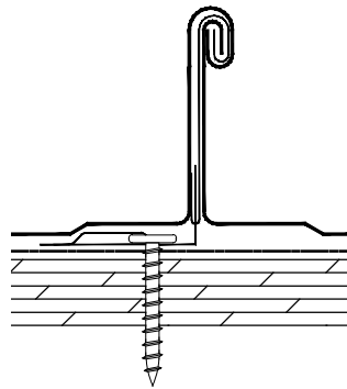
180° SEAM
