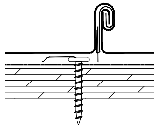
180° SEAM
