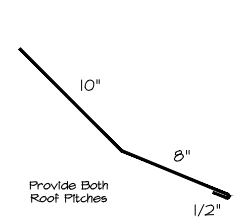
(20a) TRANSITION HIGH LOW
