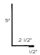
(10a) SIDEWALL
