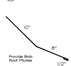
20a TRANSITION HIGH LOW
