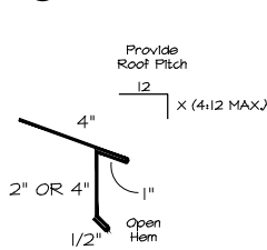
5c STYLE D EAVE
