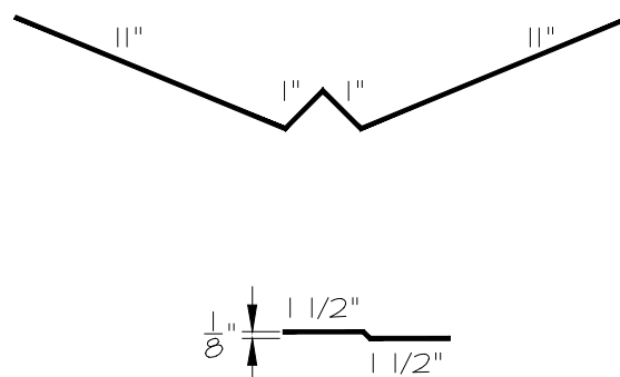
24" W-Valley
