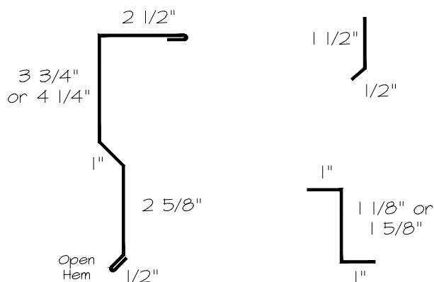
2x6 Gable
