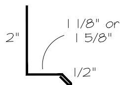
Base Trim
