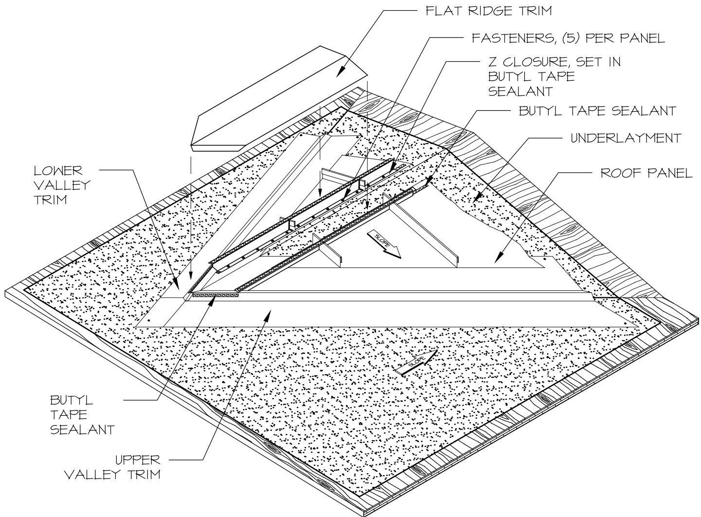
Dormer Tie-In
