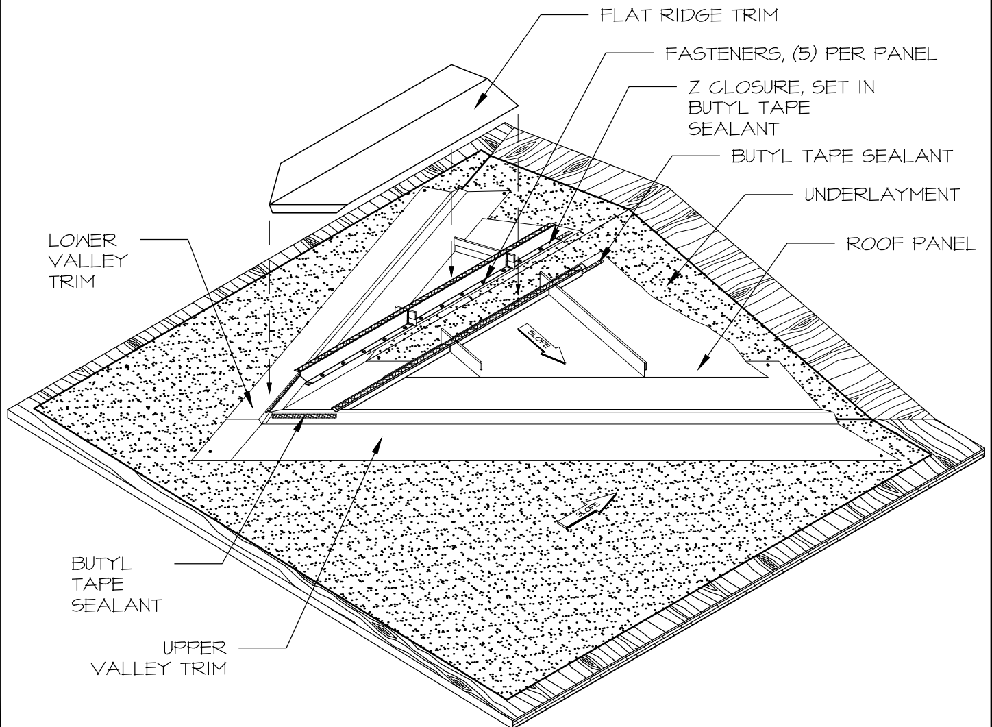
Dormer Tie-In
