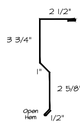
(10a) SIDEWALL
