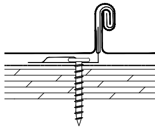
180° SEAM
