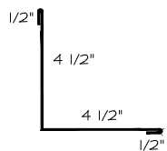
(14) INSIDE CORNER
