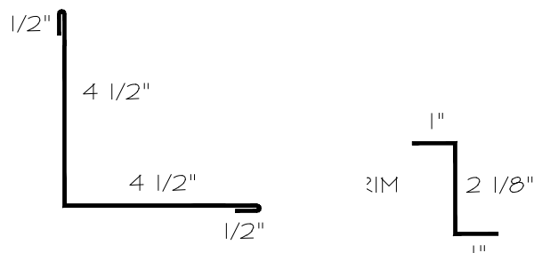
Inside Corner
