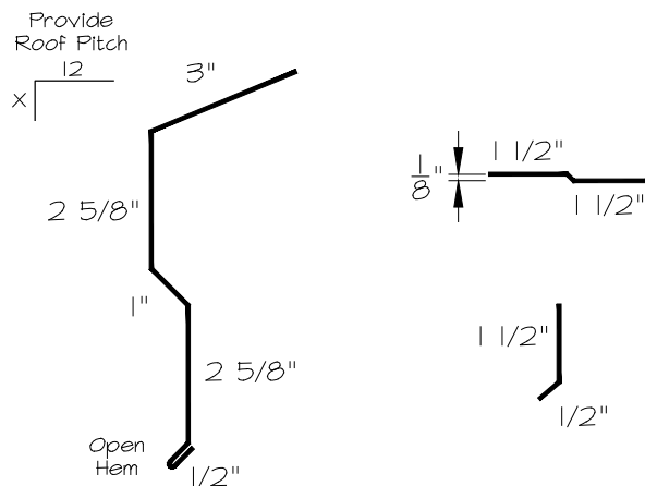
2x6 Eave
