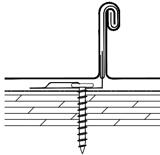
180° SEAM
