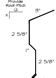
20a) TRANSITION HIGH LOW
