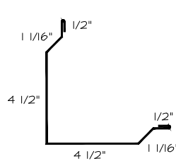
15) OUTSIDE CORNER
