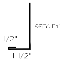
Fascia 10'-2\" Pcs.
