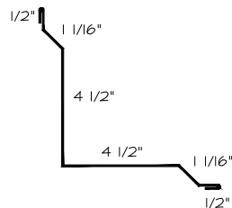
11 SNOW BREAK
