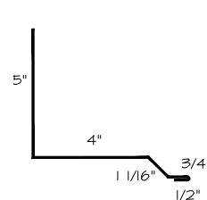
10 SIDEWALL
