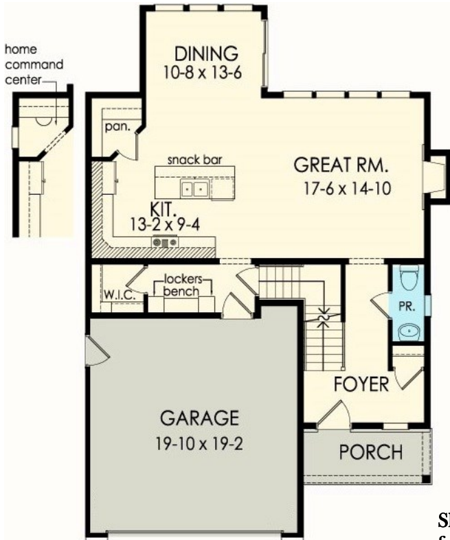
FIRST FLOOR 875 SF
