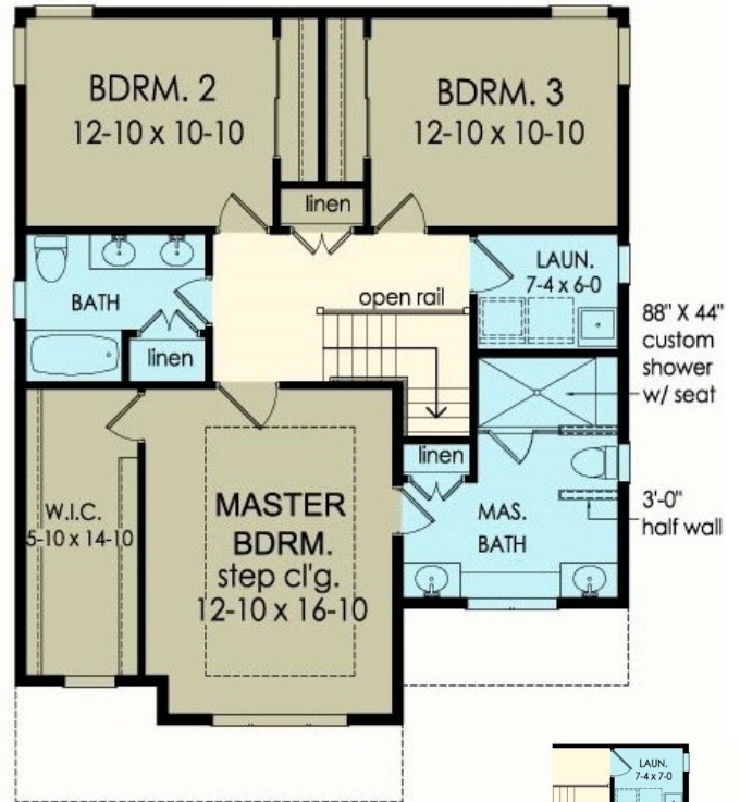
SECOND FLOOR 1077 SF
