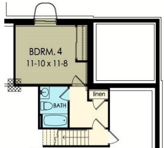
ALT - 4th BR Layout (Adds 348 SF)
