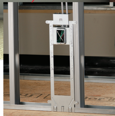
Floor-Mounted Assemblies
