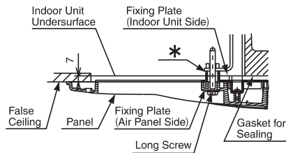
Fig. 2.3 Cross Section of Air Panel
