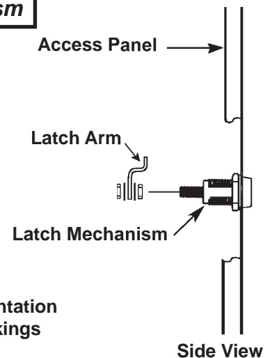
Mounting Latch
