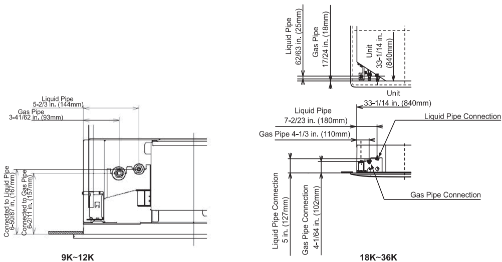
Fig.4.1 Position of Piping Connection
