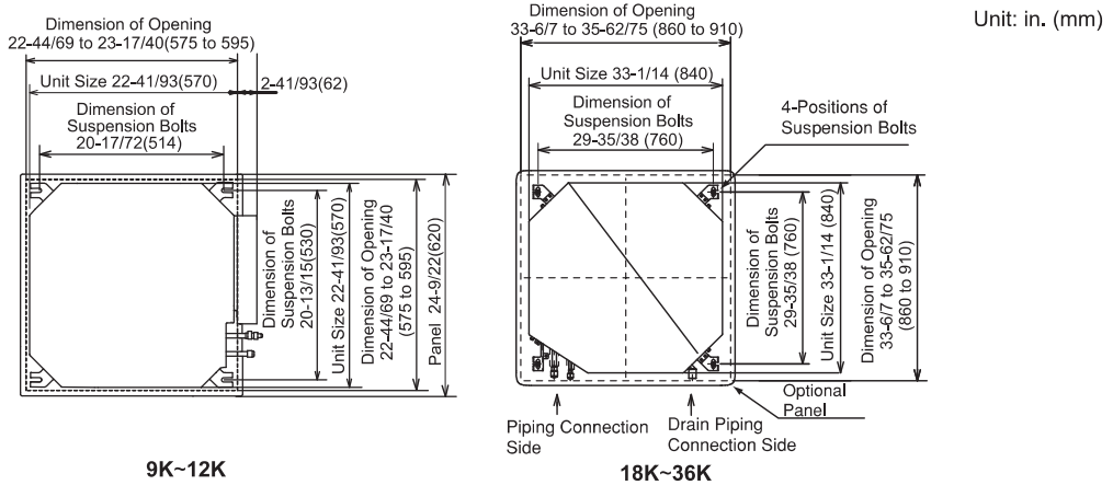
Fig.3.3 Opening of False Ceiling and Suspension Bolts
