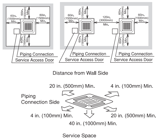
Fig. 3.1 Space around Indoor Unit
