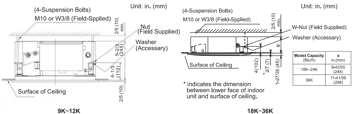
Fig. 3. 5 Mounting Position
