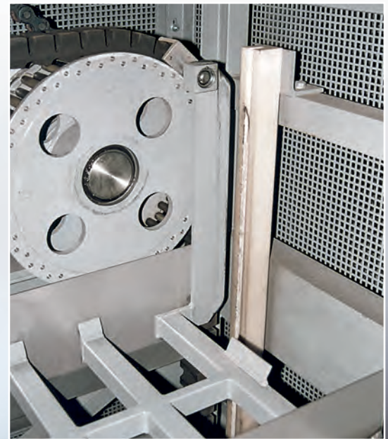
Driven wheel, plastic guide rail and platform of a circulating vertical conveyor for unit loads of varying dimensions.
