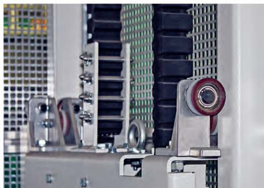
Vulkollan rollers guide the carriage
