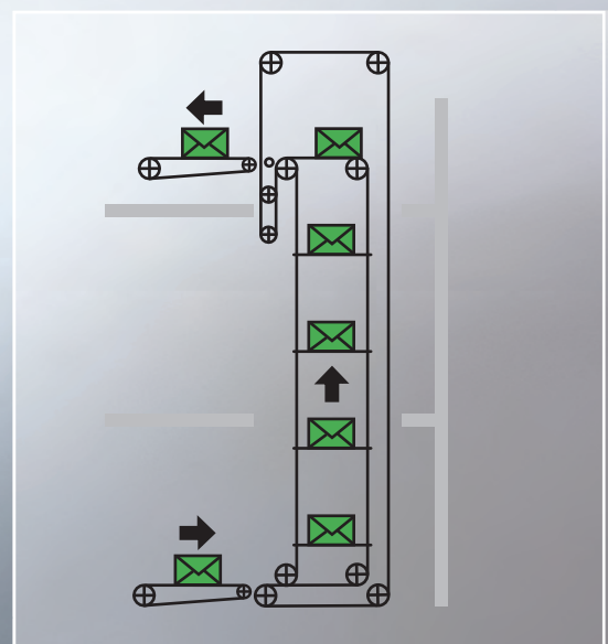
With the C-type conveyor, the feed and discharge point are on the same side. At the feed station, the item is conveyed by the reversing platform strand.
