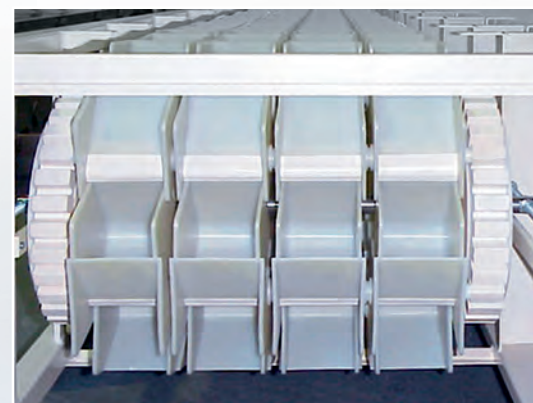
Multiple bucket belt at the tensioning unit
