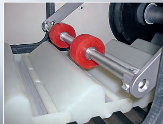
Pendulum bucket knocker to assist product discharge
