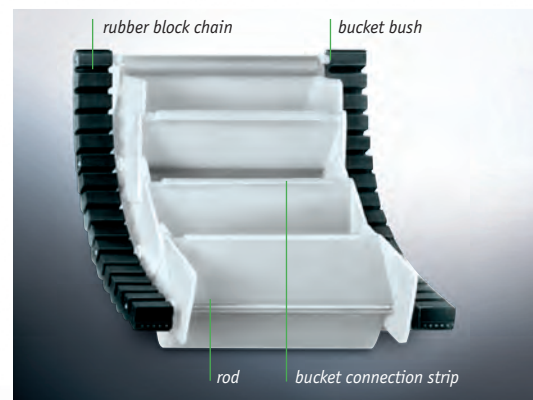
Bucket belt components and rubber block chain
