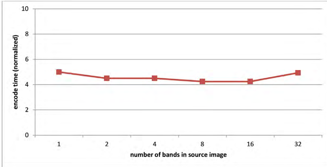
Figure 1a: Time to encode an image with a varying numbers of bands
