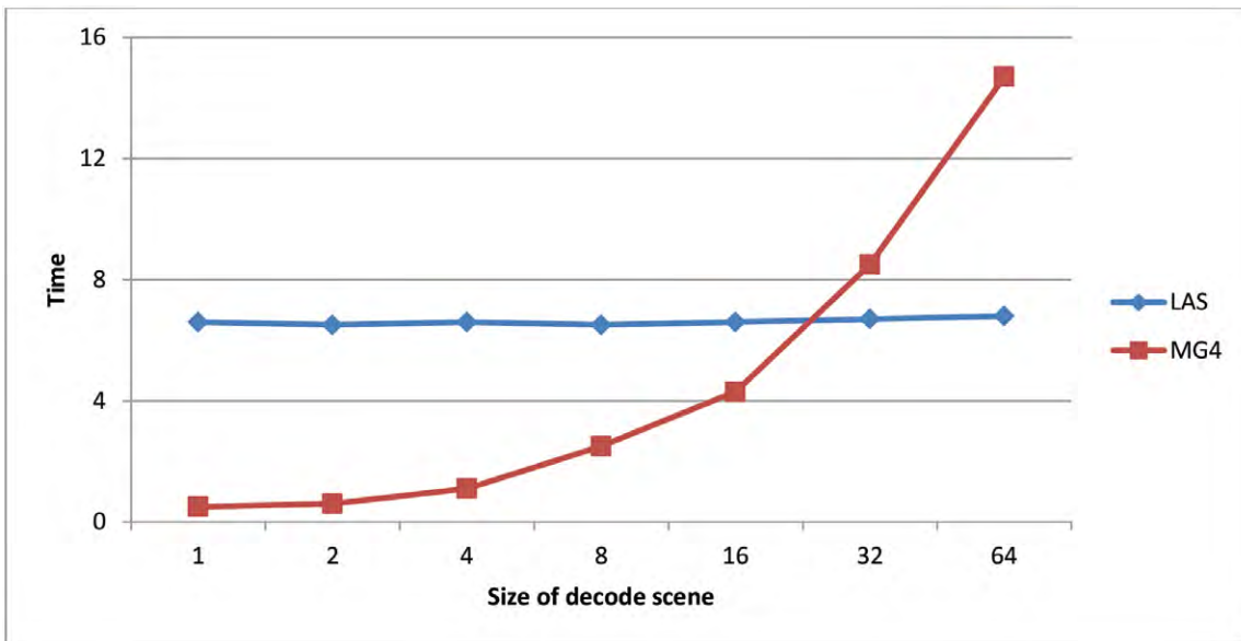
Figure 1b: Time to decode an image with a varying numbers of bands
