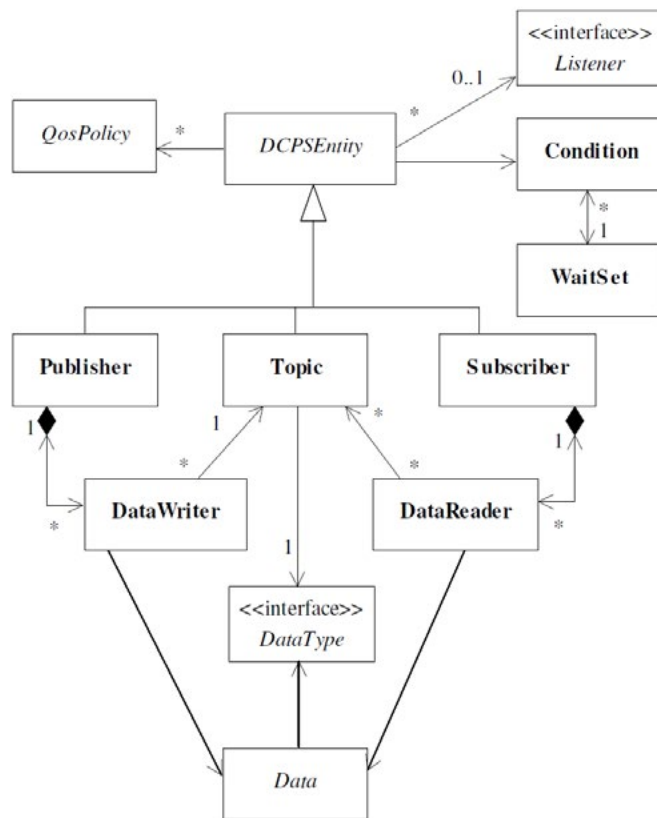
Figure 1. UML diagram of the DCPS model
